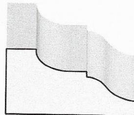
TS-CO 26 1 1/2 X 3/4
